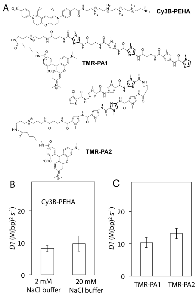
Figure 3. Molecular sled activity of synthetic small molecules. A) Chemical structures of Cy3B-PEHA, TMR-PA1 and TMR-PA2. DNA is colored by electrostatic potential. B) The D1 values of Cy3B-PEHA in 2 mM NaCl and 20 mM NaCl buffers. C) The D1 values of TMR-PA1 and TMR-PA2 in 2 mM NaCl buffer. See the Supporting Information, Table S5 for D1 values.
