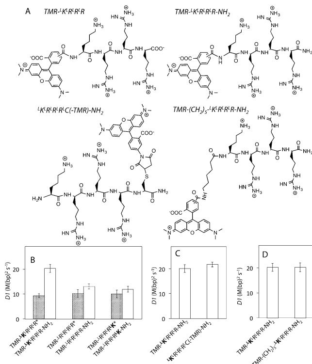
Figure 1. A) Selected chemical structures. B–D) One-dimensional diffusion constants (D1) of peptidyl sleds in 2 mM NaCl buffer (all buffers are pH 7.4). TMR was conjugated to the N-terminal amines of all peptides except for L K L R L R L R L C-(TMR)-NH 2 . Error bars represent 95% confidence intervals in all figures. * Indicates data that were previously published [4] and re-analyzed here. See the Supporting Information, Table S2 for D1 values.
